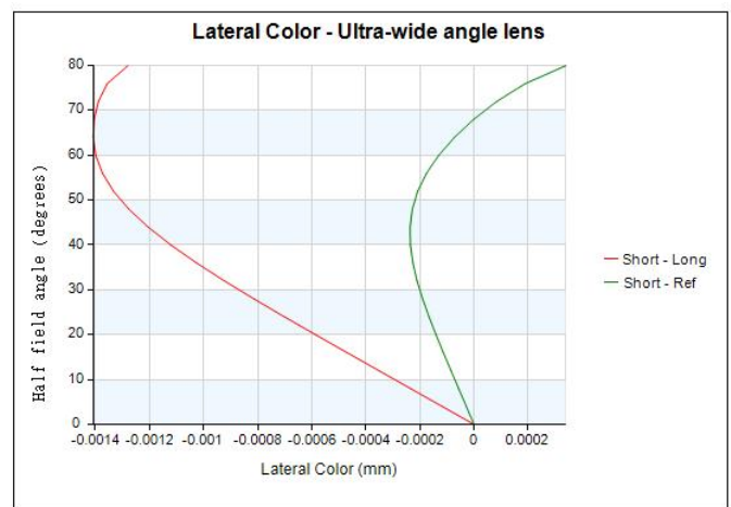
FIG. 8 Lateral color for the ultra-wide angle lens design.
