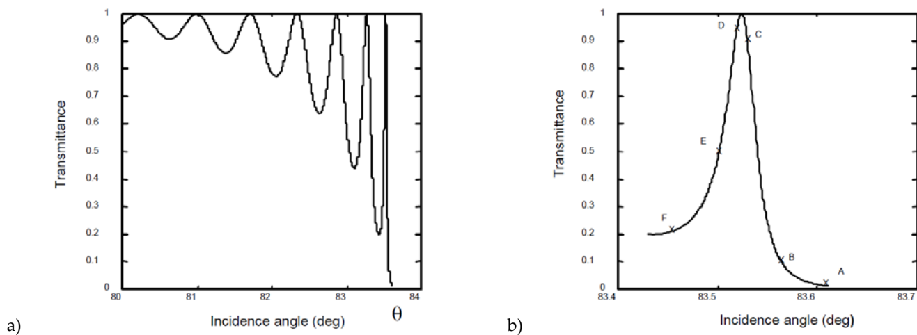
FIG. 2a) Linear optical transmittance ( n_2 l \sim 0 ) near the critical angle ( \theta_c \sim 83.61^\circ ). b) Magnification of the last peak of ( T ) in 2a).
