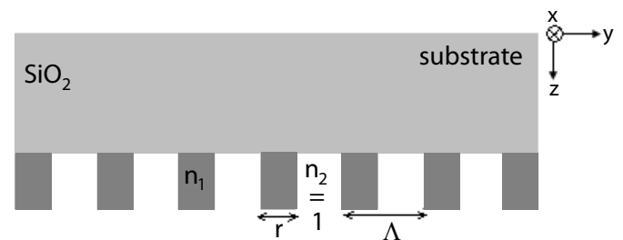
FIG. 4 Short period phase mask with corrugation in a high index layer on silica for tolerant extinction of the 0 th transmitted order.
