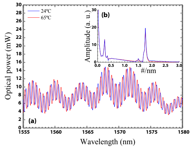
FIG. 6 Experimental results of the RI tip sensor when temperature was applied for 24°C and 65°C, respectively, for (a) spectral response and (b) FFT analysis.
