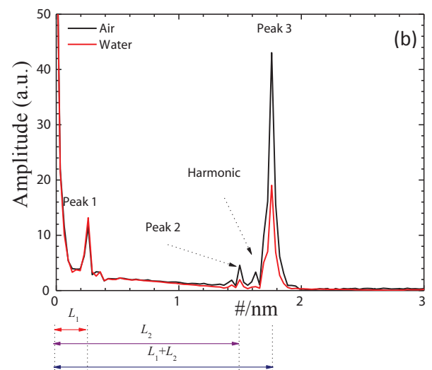
FIG. 2 (a) Spectral response when the sensing head is in the air and in the water, respectively. (b) FFT result of the two spectral responses.
