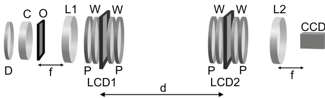
FIG. 1 Sketch of the anamorphic zoom system. D is a diffuser, C a condenser lens, O the object, L_1 and L_2 are lenses, W s and P s are waveplates and polarizers respectively, LCD_1 and LCD_2 are liquid crystal displays and CCD is a detector.
