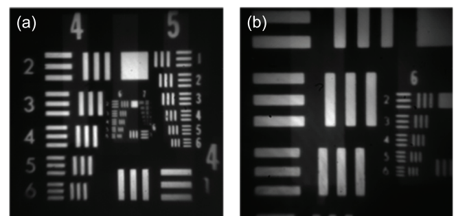
FIG. 2 Two images obtained by displaying onto the SLMs spherical lenses with variable focal length. The zoom factor between a) and b) is approximately 2.
