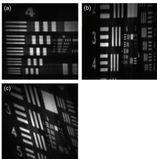
FIG. 3 Distortions introduced by means of the anamorphic lenses: a) horizontal stretching, b) vertical stretching and c) diagonal stretching.
