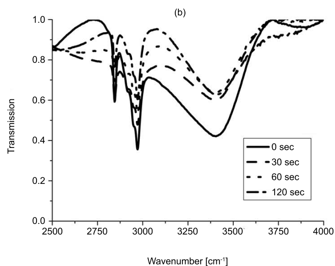
FIG. 3 FTIR transmission of fast sol-gel at different UV-curing times in two absorption regions, 400 - 1800\text{ cm}^{-1} (a) and 2500 - 4000\text{ cm}^{-1} (b).
