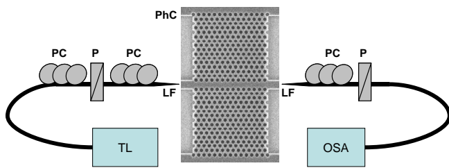
FIG. 1 Schematic of setup employed and SEM image of a 5 \mu\text{m} photonic crystal waveguide inserted as the PhC. The actual sample used was 50 \mu\text{m} in length but with identical crystal parameters. Also not shown because of size restraints in the imaging process is the SOI tapered input waveguides leading into the structure. PhC - photonic crystal; PC - polarisation controller; P - polariser; LF - lensed fibre; TL - tuneable laser; OSA - optical spectrum analyser.
