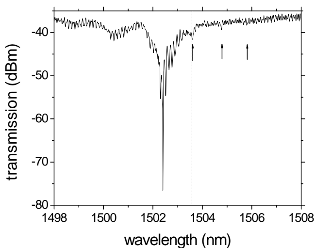
FIG. 3 Transmission resonant notch spectra optimised to have quasi- TE at wavelengths below and quasi- TM at wavelengths above the quasi- TE transmission band edge. Arrows point out additional resonant peaks.
