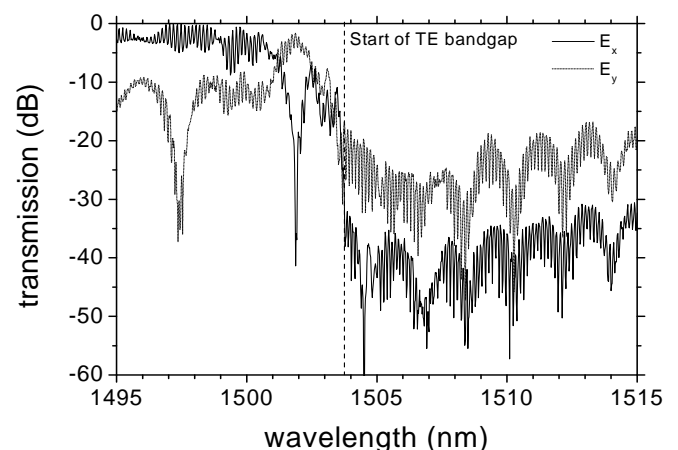
FIG. 2 Transmission spectra of quasi- TE and TM fields through the device. Narrow transmission gap is observed at 1502 nm for TE light. A corresponding rise in TM signal is seen.
