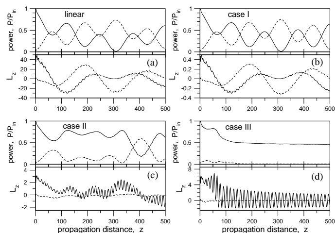
FIG. 2 Power (normalised) and angular momentum L_z versus propagation distance for each of the cores of the PCF coupler, when a vortex is launched into one of the cores. The continuous line corresponds to the initially excited core (first core) and the dashed line to the second core. (a) Linear propagation regime. (b-d) Nonlinear regime for different input powers corresponding to the simulations showed in Figure 1 (labels I, II and III are correspondent in both figures). Input powers: P_I = 0.5 , P_{II} = 3 and P_{III} = 6 .
